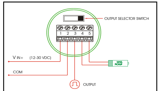
Model PET-5 0-10 VDC Square Pulse
