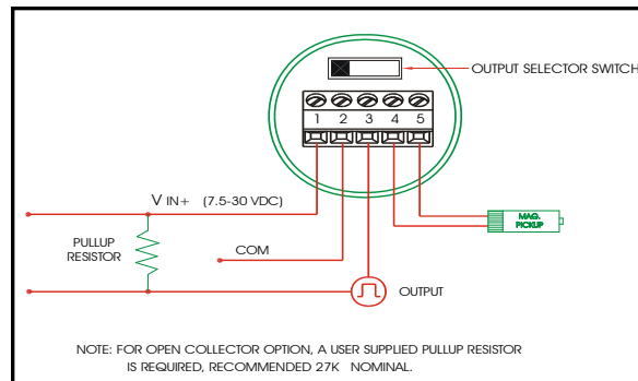
Model PET-6 Open Collector
